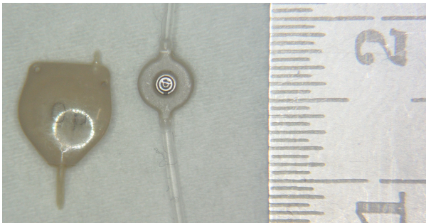
Photograph showing the real size comparison between the eyeWatch (left) and the Stergio Valve (right)
