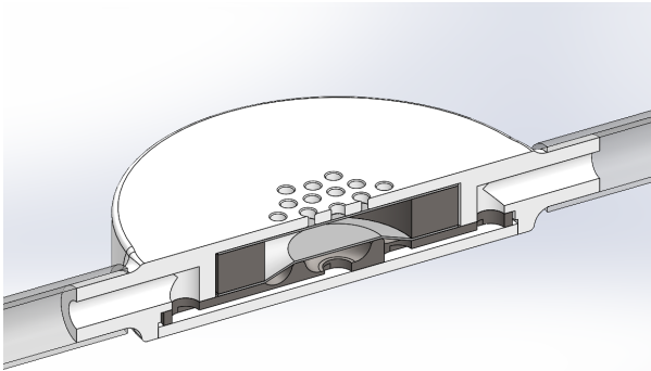
Schematic drawing of the Stergio Valve mechanism
